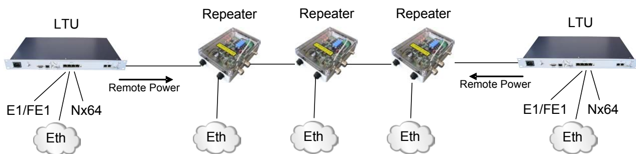
Ethernet Add/Drop Repeater Application with Remote Power
