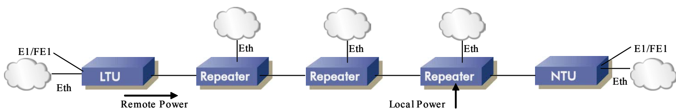
Ethernet Add/Drop Repeater Application with Remote Power
